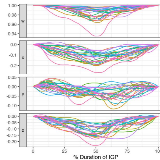
eGait device and IGPs of 27 patients diagnosed with multiple sclerosis
